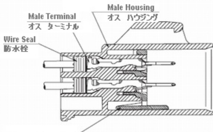
Male Pre-set Secondary Terminal Lock (TPA) オス側 事前組付け二重係止板
