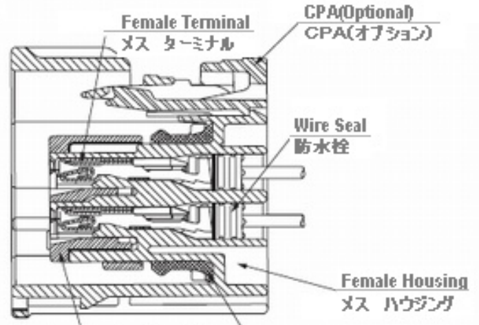
Female Pre-set Secondary Terminal Lock(TPA) メス側 事前組付け二重係止板
