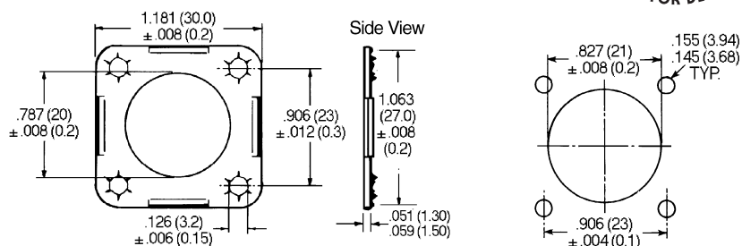
Mounting Dimensions
