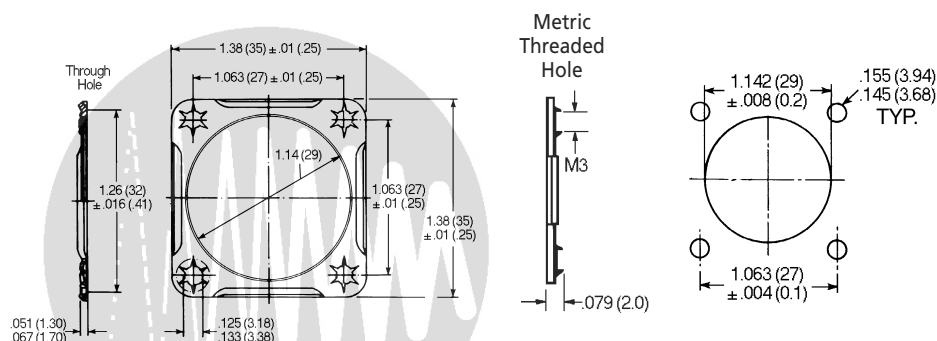
Mounting Dimensions
