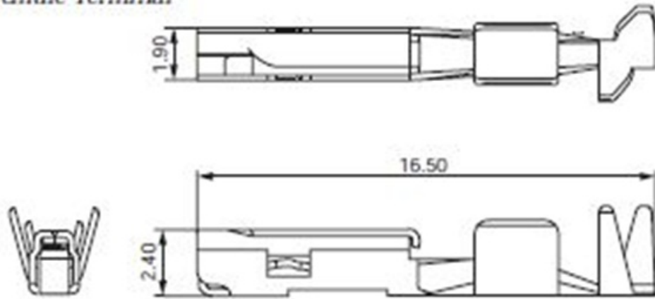
Female Terminal
