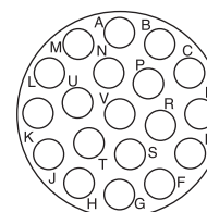
Shell Size 16 0 Power 19 Signal
