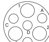
Shell Size 14 3 Power 4 Signal
