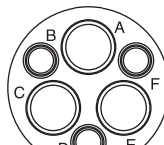
Shell Size 14 3 Power 3 Signal
