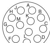
Shell Size 14 0 Power 12 Signal
