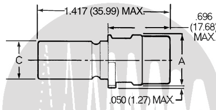
Plug
