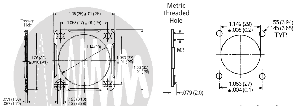
Mounting Dimensions
