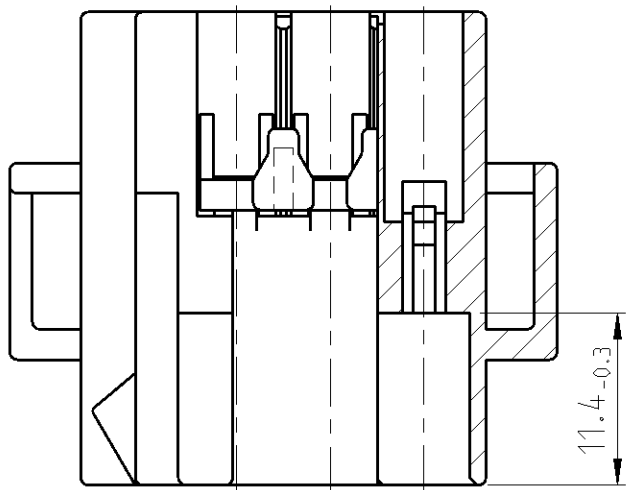
Section B-B SECTION
